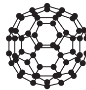
C_{60} fullerene
